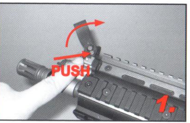
1. 按下左側卡筭鈕，準星方能立起或向前摺疊 Push the button on left of front sight to fall or stand the front sight.
